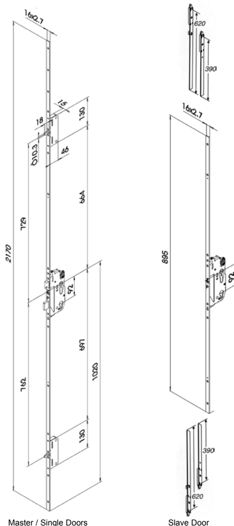
Master / Single Doors
